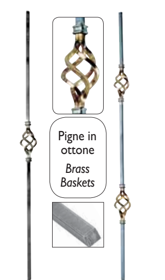
Art. 1149/1 Art. 1149/2 Ø 12 x 12 mm Ø 12 x 12 mm H 1000 mm H 1000 mm
