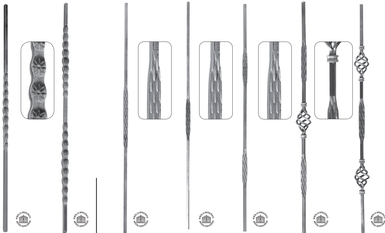
Art. 1718/9 Art. 1718/11 Art. 1727/1 Art. 1729/11 Art. 1727/3 Art. 1729/3 Art. 1729/1 Φ 12 × 12 mm Φ 12 × 12 mm Φ 12 × 12 mm Φ 12 × 12 mm Φ 12 × 12 mm Φ 12 × 12 mm Φ 12 × 12 mm H 1000 mm H 1000 mm H 1000 mm H 1000 mm H 1000 mm H 1000 mm H 1000 mm Art. 1718/10 Art. 1718/12 Art. 1727/2 Art. 1729/12 Art. 1727/4 Art. 1729/4 Art. 1729/2 Φ 14 × 14 mm Φ 14 × 14 mm Φ 14 × 14 mm Φ 14 × 14 mm Φ 14 × 14 mm Φ 14 × 14 mm Φ 14 × 14 mm H 1000 mm H 1000 mm H 1000 mm H 1000 mm H 1000 mm L 55 mm L 55 mm H 1000 mm H 1000 mm L 55 mm L 55 mm
