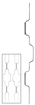
Art. 142/2 20 x 4 mm H 800 mm
