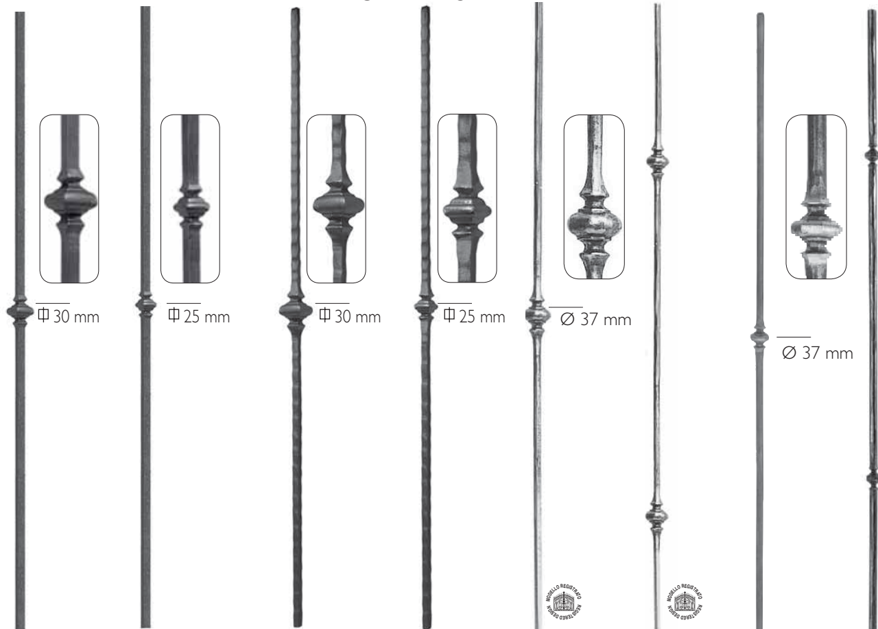
Art. GD248/1 Φ 12 x 12 mm H 1000 mm Art. GD248/2 Φ 12 x 12 mm H 1000 mm Art. GD248/3 Φ 12 x 12 mm H 1000 mm Art. GD248/4 Φ 12 x 12 mm H 1000 mm Art. 499/1 Ø 12 mm H 1000 mm Art. 499/2 Ø 12 mm H 1000 mm Art. 1770/3 Ø 12 mm H 1000 Art. 1771/3 Ø 12 mm H 1000
