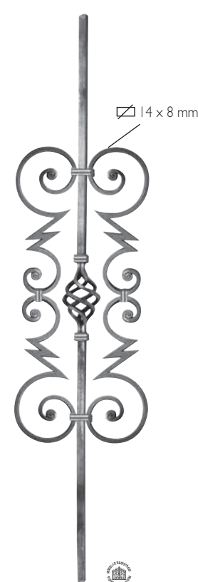
Art. GDI96/3 \Phi 14 x 14 mm H 1000 mm L 215 mm
