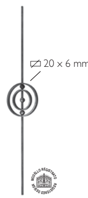
Art. 1082/1 Ø 10 mm H 1000 mm L 160 mm
