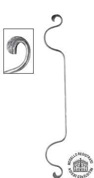
Art. 1303/3 Ø 10 mm H 800 mm L 105 mm
