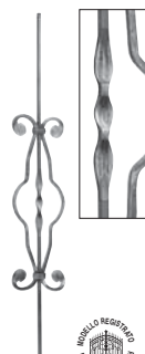
Art. 586/3 Ø 8 x 8 mm H 900 mm L 130 mm
