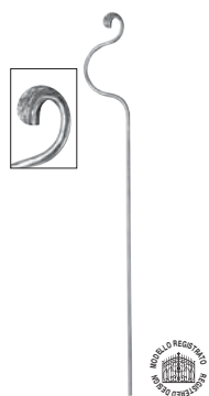
Art. 1303/1 Ø 10 mm H 830 mm L 105 mm
