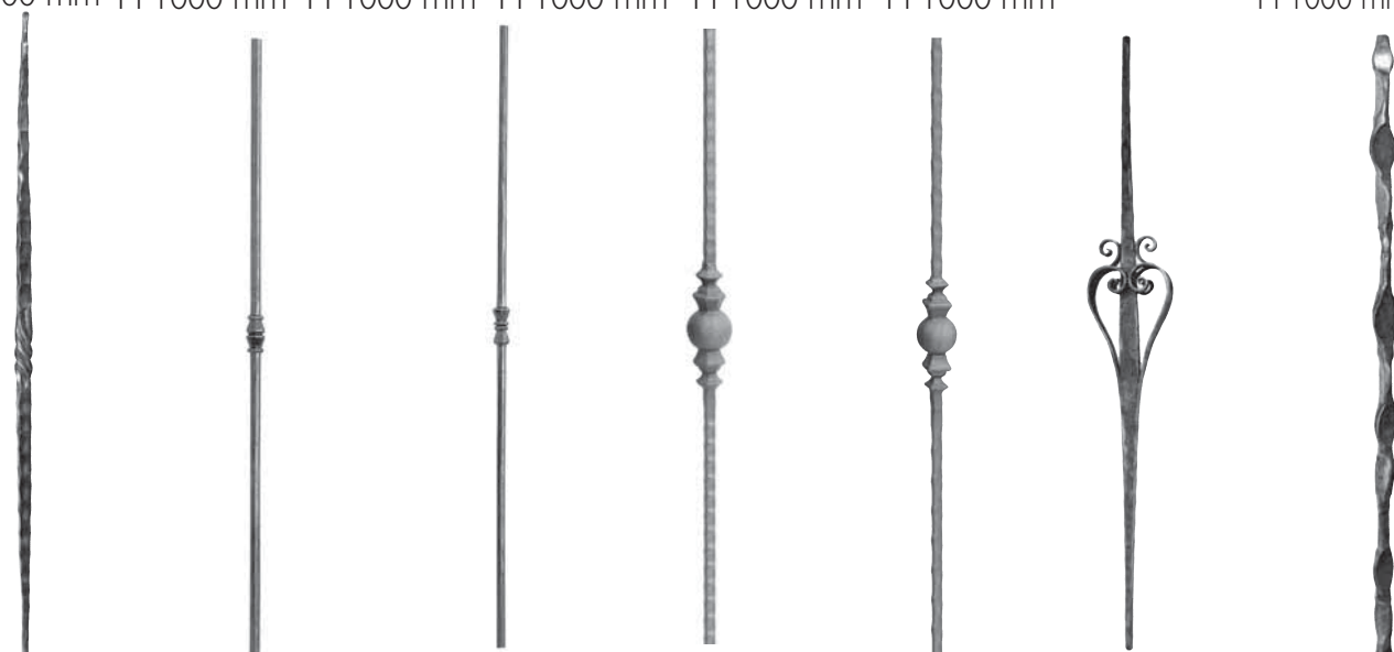
Art. 96/1 Art. 1192/8 Art. 1192/9 Art. 502/1 Art. 502/2 Art. 96/3 Art. 96/4 \Phi 20 x 8 mm \Phi 14 mm \Phi 12 mm \Phi 14 x 14 mm \Phi 14 x 14 mm \Phi 16 x 8 mm \Phi 16 x 8 mm H 830 mm H 1000 mm H 1000 mm H 1000 mm H 900 mm H 830 mm H 830 mm
