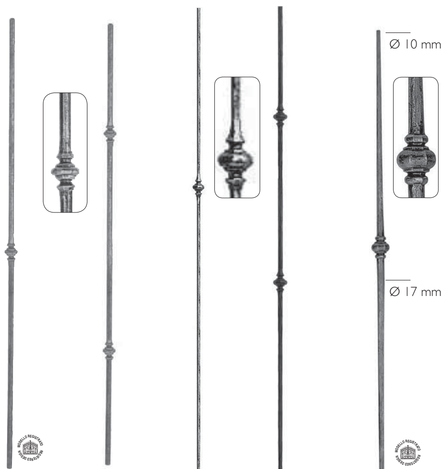
Art. 1770/2 Ø 12 mm H 1000 mm Art. 1771/2 Ø 12 mm H 1000 mm Art. 1159/1 Ø 12 mm H 1200 mm Art. 1159/2 Ø 12 mm H 1200 mm Art. 1184/5 H 1000 mm Conico/Conic
