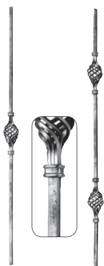
Art. 48/B/6 Art. 48/B/5 Ø 12 x 12 mm Ø 12 x 12 mm H 900 mm H 900 mm L 55 mm L 55 mm
