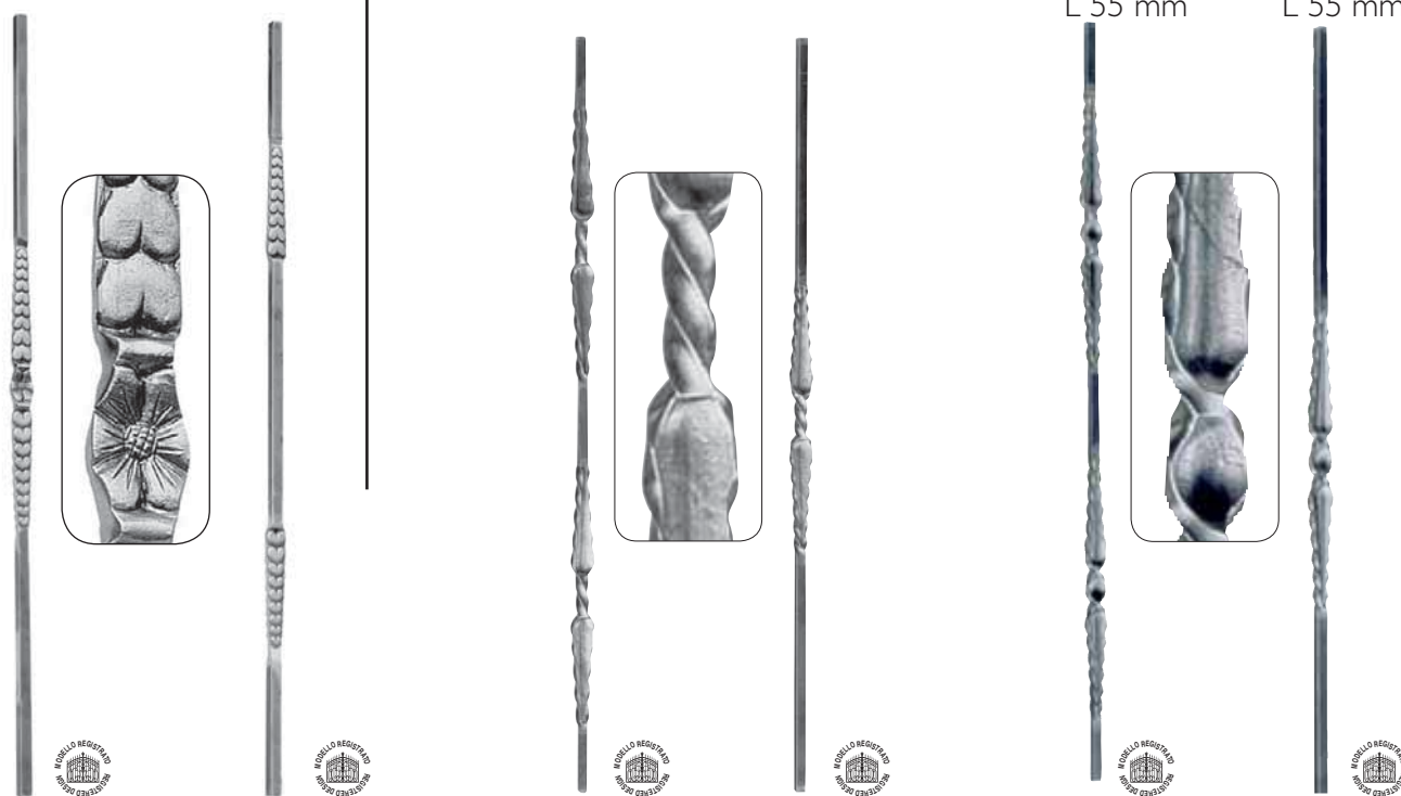
Art. 1718/13 Art. 1718/15 Art. 1730/1 Art. 1730/3 Art. 1730/5 Art. 1730/7 Φ 12 × 12 mm Φ 12 × 12 mm Φ 12 × 12 mm Φ 12 × 12 mm Φ 12 × 12 mm Φ 12 × 12 mm H 1000 mm H 1000 mm H 1000 mm H 1000 mm H 1000 mm H 1000 mm Art. 1718/14 Art. 1718/16 Art. 1730/2 Art. 1730/4 Art. 1730/6 Art. 1730/8 Φ 14 × 14 mm Φ 14 × 14 mm Φ 14 × 14 mm Φ 14 × 14 mm Φ 14 × 14 mm Φ 14 × 14 mm H 1000 mm H 1000 mm H 1000 mm H 1000 mm H 1000 mm H 1000 mm
