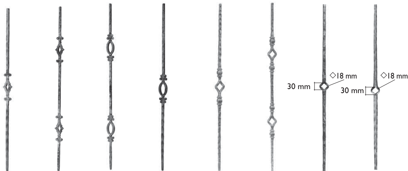
Art. 489/2 Art. 489/1 Art. 490/1 Art. 490/2 Art. 507/1 Art. 507/2 Art. 101/2 Art. 101/1 \Phi 12 x 12 mm \Phi 12 x 12 mm \Phi 12 x 12 mm \Phi 12 x 12 mm \Phi 14 x 14 mm \Phi 14 x 14 mm H 1000 mm \Phi 14 x 14 mm H 1000 mm H 1000 mm H 1000 mm H 1000 mm H 1000 mm H 1000 mm H 1000 mm
