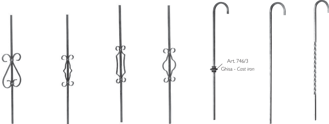
Art. 1128/2 \varnothing 12 x 12 mm H 1000 mm L 195 mm
