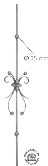
Art. 1060/3 Ø 12 mm H 1000 mm L 190 mm
