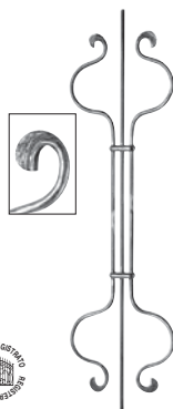
Art. 1075/2 Ø 10 mm H 1000 mm L 245 mm
