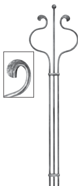
Art. 1075/1 Ø 10 mm H 1000 mm L 245 mm
