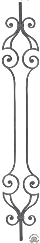
Art. GDI50/2 \Phi 14 x 14 mm H 1000 mm L 205 mm
