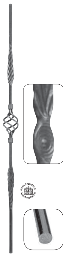
Art. 1734/1 \varnothing 12 mm H 1000 mm L 55 mm
