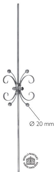
Art. 1061/1 Ø 12 mm H 1000 mm L 205 mm
