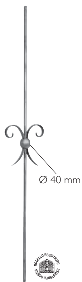
Art. 1060/1 Ø 12 mm H 1000 mm L 165 mm
