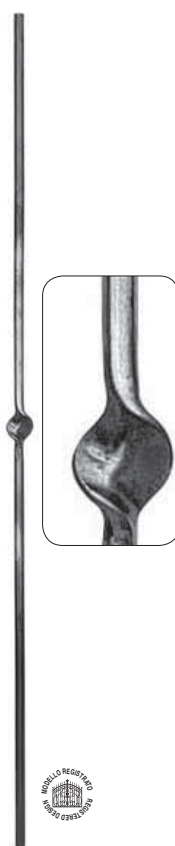
Art. 1067/1 \varnothing 12 mm H 1000 mm
