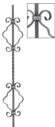
Art. 1127/2 \varnothing 12 x 12 mm H 1000 mm L 160 mm
