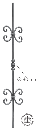
Art. 1064/2 Ø 12 mm H 1000 mm L 175 mm
