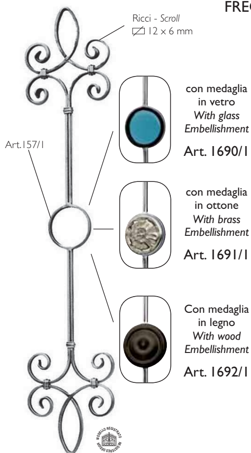
Art. 1688/5 \nabla 12 x 12 mm H 1000 mm L 200 mm
