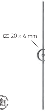
Art. 1082/3 Ø 10 mm H 1000 mm L 100 mm
